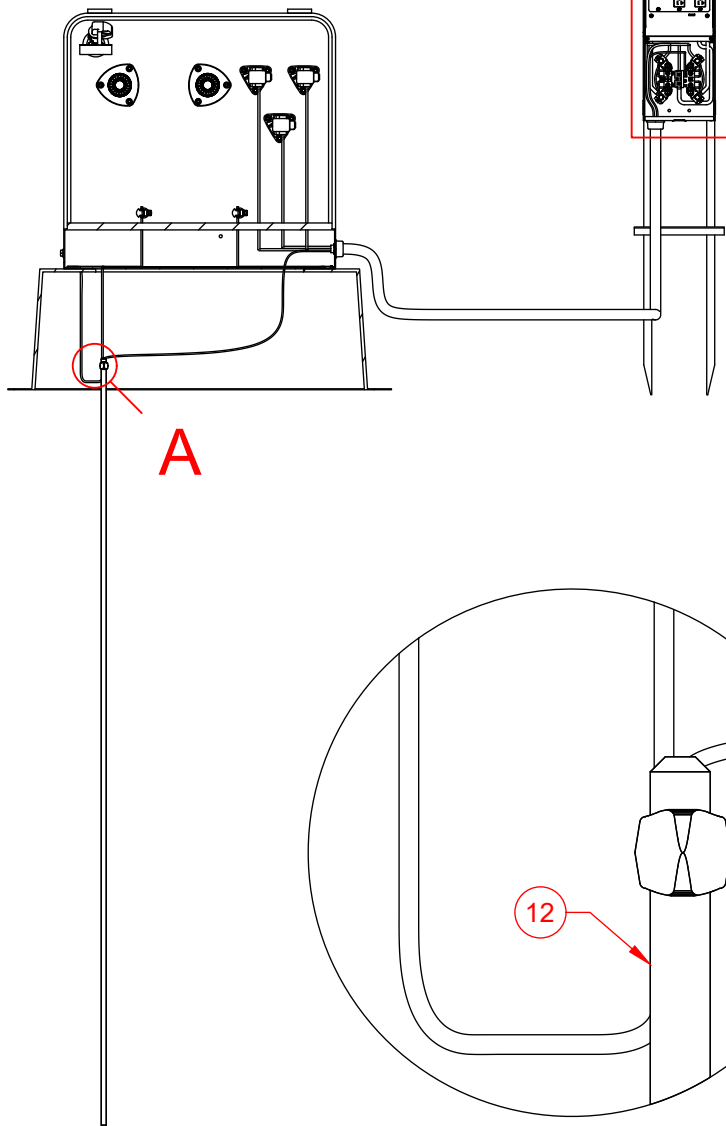
DETAIL A (GROUNDING) SCALE 1:2
