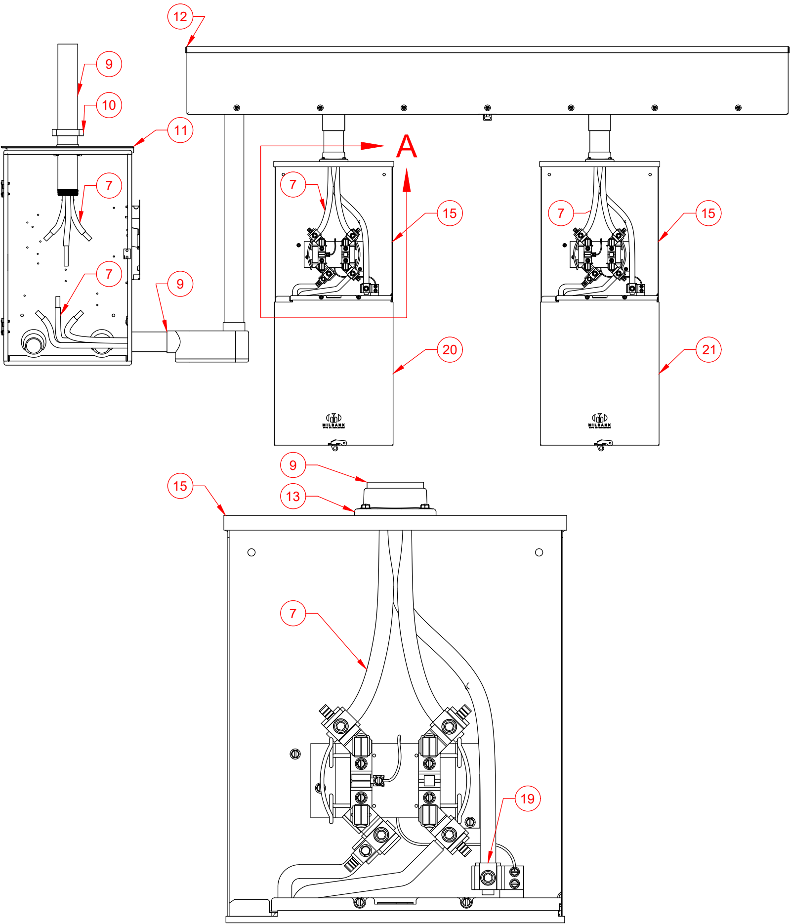
DETAIL A SCALE 1:4
